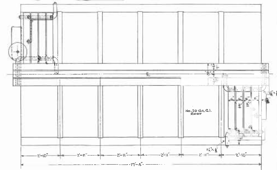
PLAN OF ROOF MURPHY PIVOTED SOLID STEEL ROOF INTERMEDIATE PANELS STANDARD, END PANELS & END RIDGE CAPS, SPECIAL.
