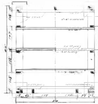
FRAMING PLAN.
