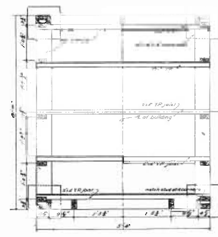
FRAMING PLAN.
