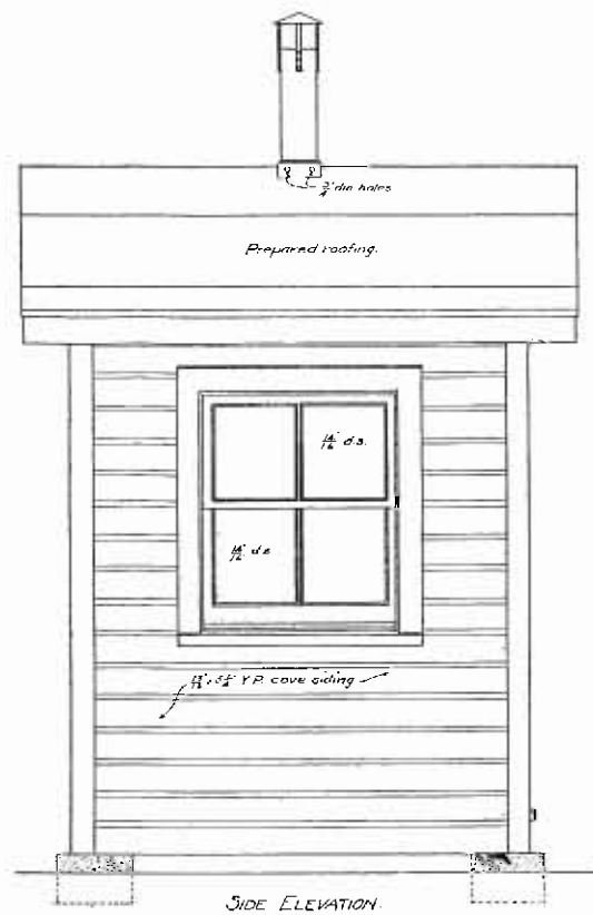
SIDE ELEVATION.
