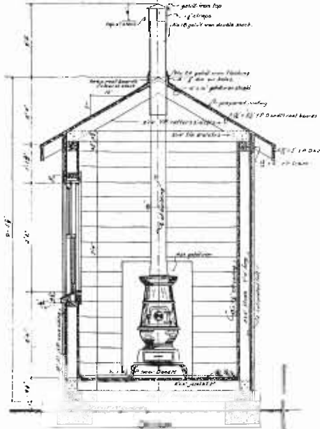
SECTION.
